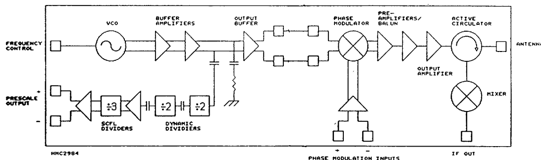
Figure 3. Single-Chip Radar MMIC Block Diagram
