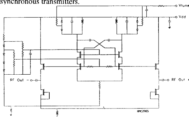
Figure 5. Schematic Diagram of VCO Circuit
