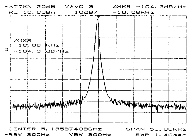
Figure 6. Transmitter Residual Sideband Noise Levels
